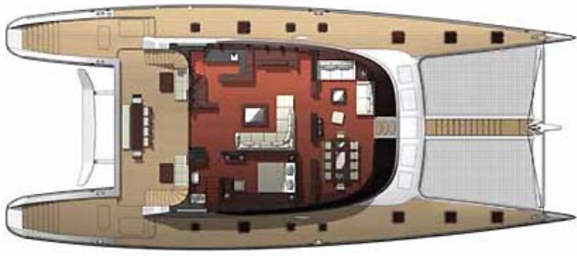
BB 100 "ALLPES" MAIN DECK ARRANGEMENT
